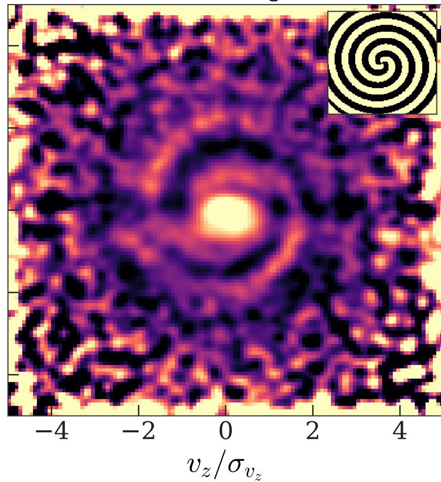
m = 2 breathing mode
