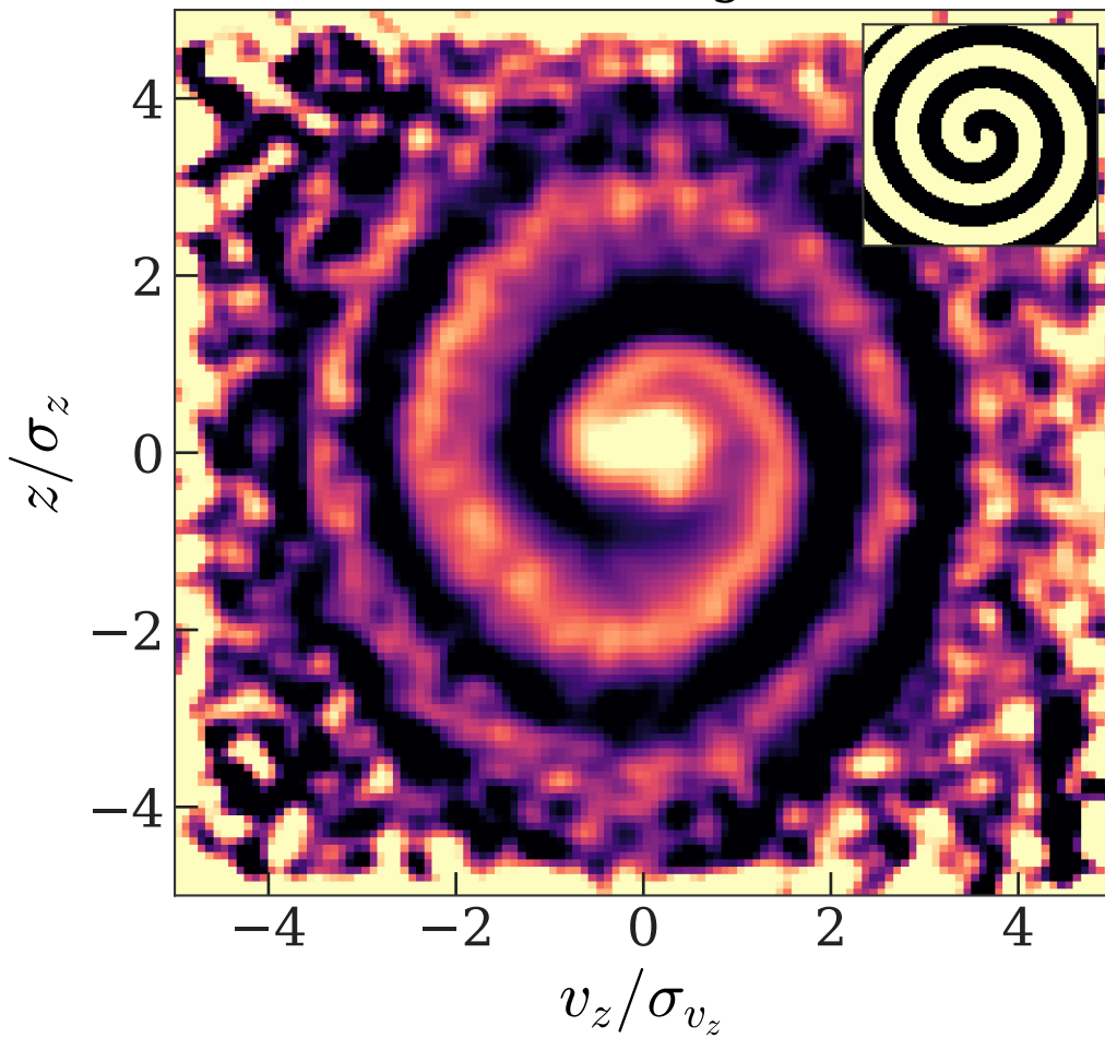
m = 1 bending mode
